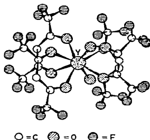
Fig. 2. The anion in \text{Cs}^+[\text{Y}(\text{CF}_3\text{COCHCOCF}_3)_4]^-
