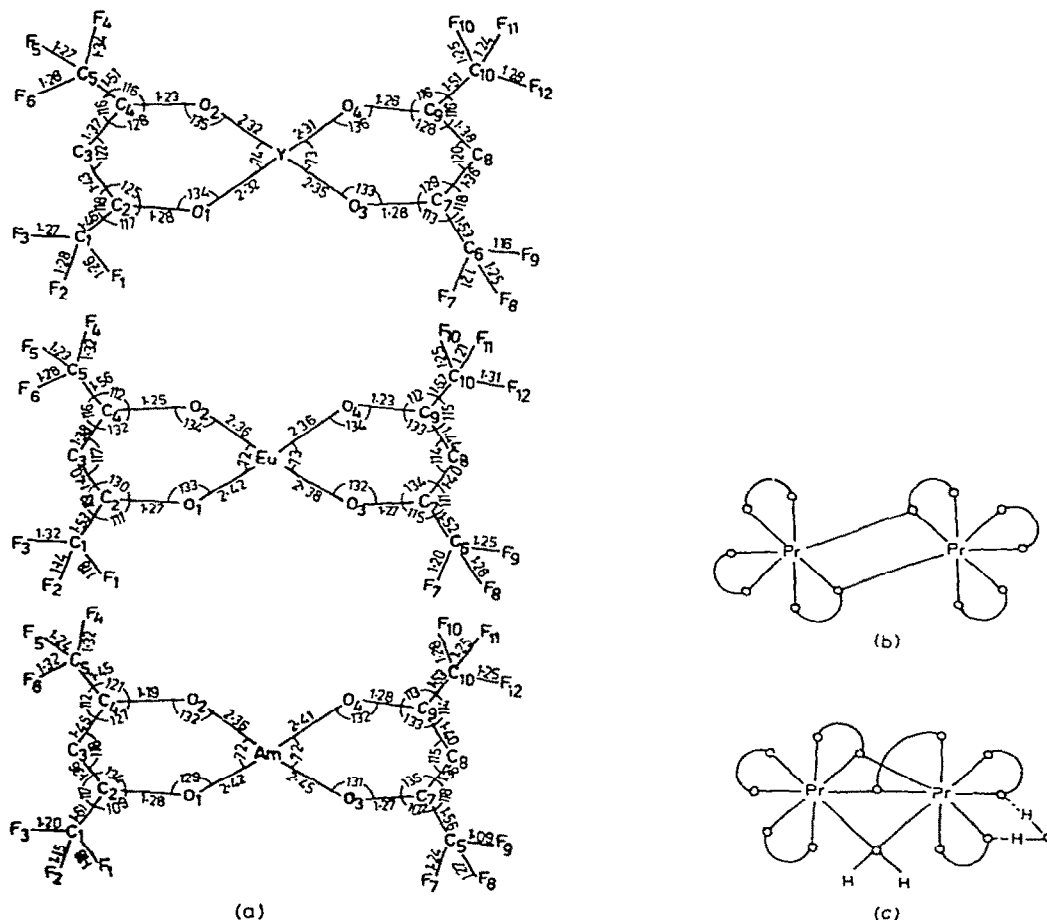
Fig. 3. (a) Comparison of bond lengths and angles in \text{Cs}[\text{Y}(\text{hfac})_4] , \text{Cs}[\text{Eu}(\text{hfac})_4] and \text{Cs}[\text{Am}(\text{hfac})_4] . (b) Schematic dimeric structure of \text{Pr}(\text{thd})_3[\text{Pr}_2(\text{thd})_6] . (c) Schematic dimeric structure of \text{Pr}(\text{fod})_3 \cdot \text{H}_2\text{O} , [(\text{fod})_3\text{Pr}(\text{OH}_2)\text{Pr}(\text{fod})_3] \cdot \text{H}_2\text{O} .
