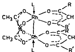
Fig. 20. Structure of [Rh(CH_3COO)(1,3\text{-Diketonato})]L_2 . L = H_2O, py, 2\text{-Cl-py}, 2\text{-Me-py} .
