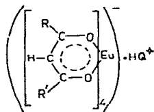
Fig. 41. R = \text{CF}_3 ; \text{R}' = ph, 1-naphthyl, 2-naphthyl, 4-MeO \cdot \text{C}_6\text{H}_4 , 2-MeO \cdot \text{C}_6\text{H}_4 , 2,5-(MeO) _2 \cdot \text{C}_6\text{H}_4 , 4-biphenyl 2-fluorenyl, 3-phenanthryl and 4-F \cdot \text{C}_6\text{H}_4 .
