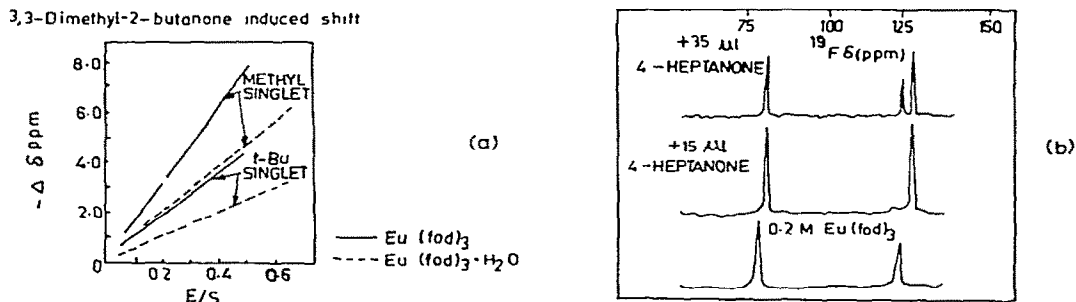
Fig. 23. (a) \Delta\delta vs. E/S for pinacolone with \text{Eu(fod)}_3 and with \text{Eu(fod)}_3 \cdot (\text{H}_2\text{O}) . (b) Anhydrous shift reagent before and after addition of 4-heptanone.
