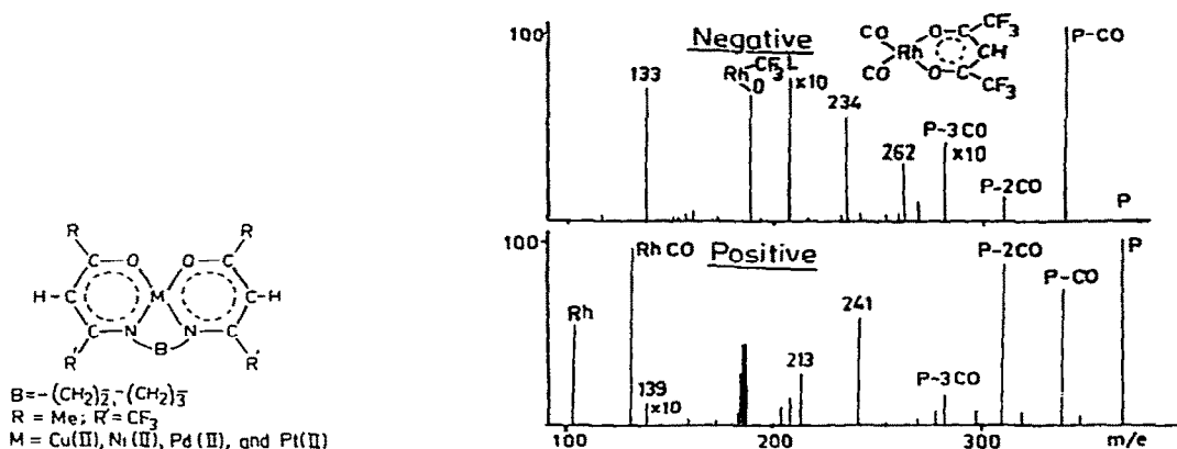
Fig. 8. Metal chelates of bis 1,3-diketone-ethylenedi-imine and its fluorinated analogues.
