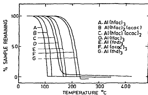
Fig. 37. Thermogravimetric curves of some volatile Al(III)-diketonates.
