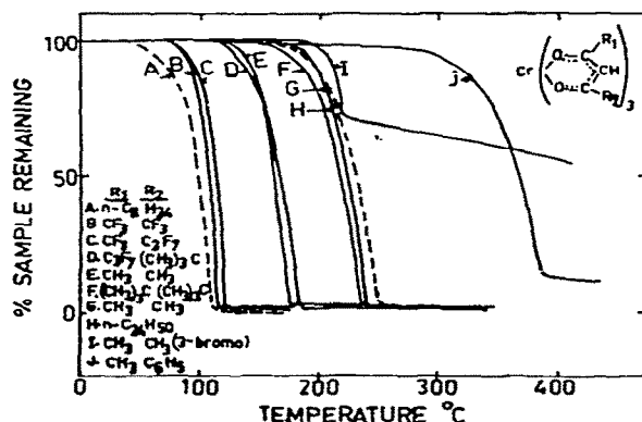
Fig. 36. Thermogravimetric curves of Cr(III) \beta -diketonates.
