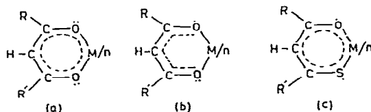
Fig. 5. Quasi-aromatic structures of metal 1,3-diketonates.
