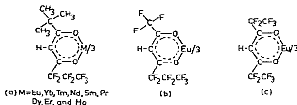
Fig. 25. (a) The nine trivalent lanthanide chelates of \text{H}(\text{fod}) . (b) The \text{dfhd} chelate of \text{Eu}(\text{III}) . (c) The \text{H}(\text{fhd}) chelate of \text{Eu}(\text{III}) .
