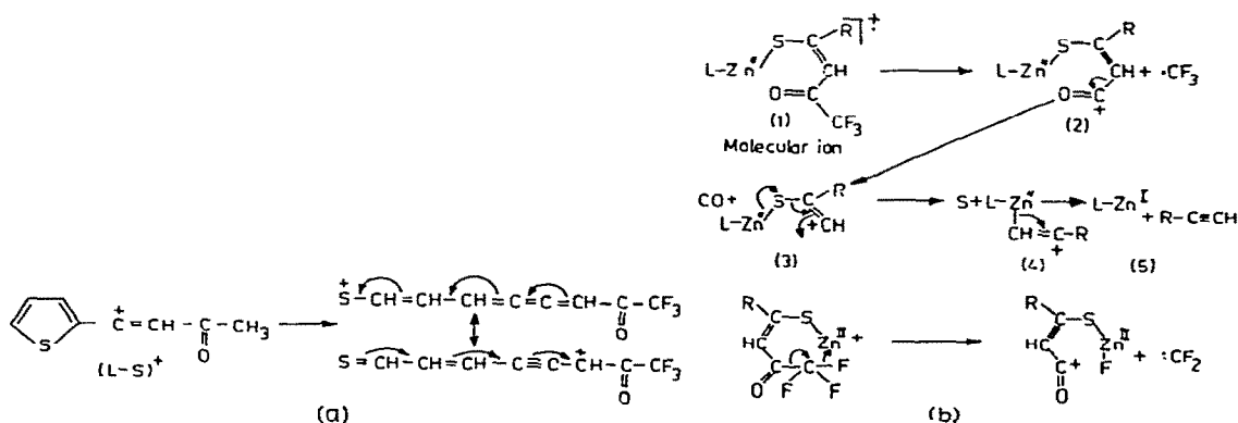
Fig. 7. (a) Resonance stabilization of the (L-S)^+ species formed by chelate of 2-thienyl ligand in the mass spectrometer. (b) Reaction of zinc chelate in the mass spectrometer.
