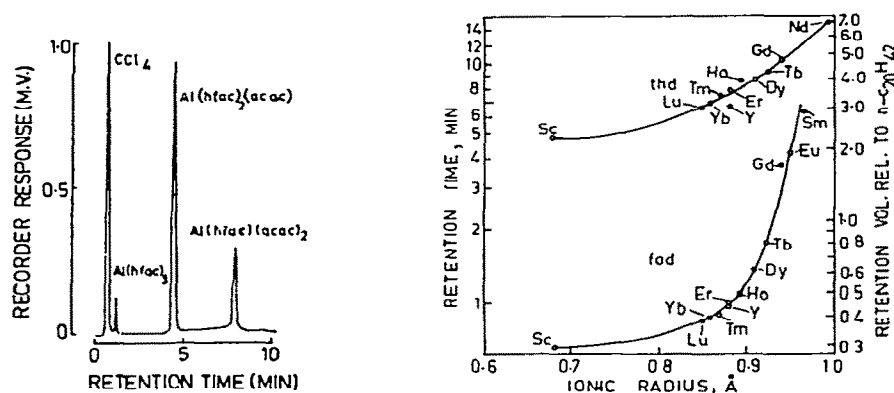
Fig. 27. Gas chromatography of metal 1,3-diketonates with degrees of substitution of hydrogen by fluorine in the ligand shell.
